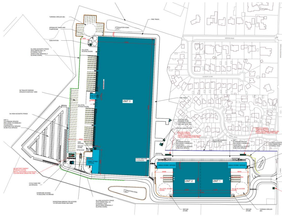
Proposed Site Plan Refer to Architects plans for latest layouts
