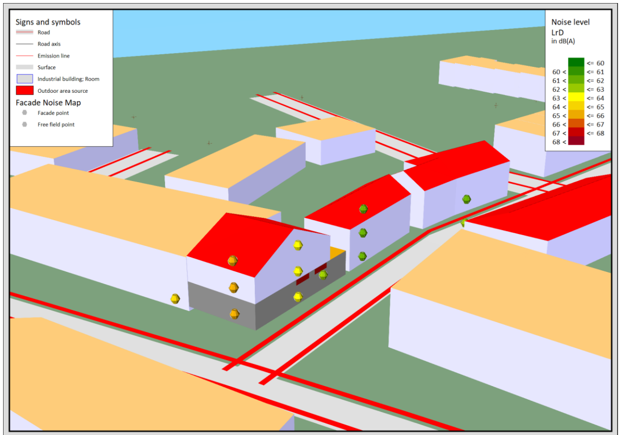
Figure 4 – Daytime FNM, 406 Manchester Road
