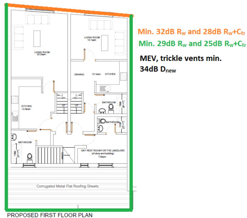
Figure 5 – Mitigation specifications for dwellings at 406 Manchester Road
