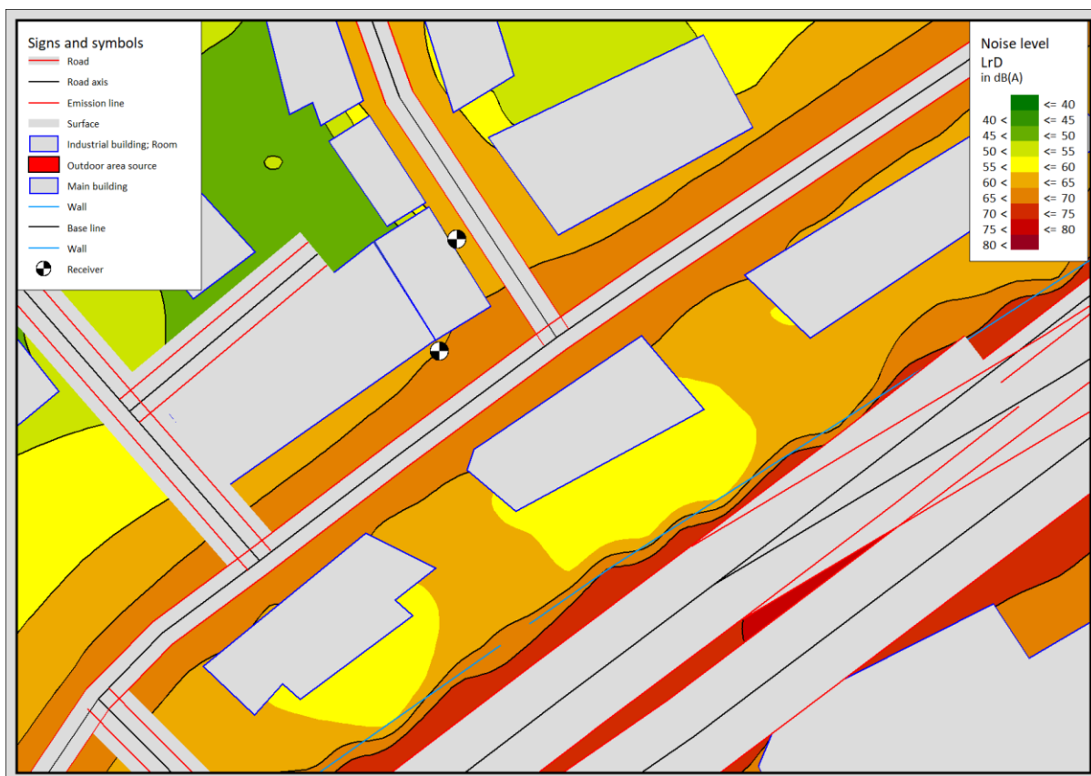
Figure 3 – Daytime GNM, 406 Manchester Road
