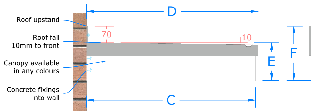
Side Elevation
