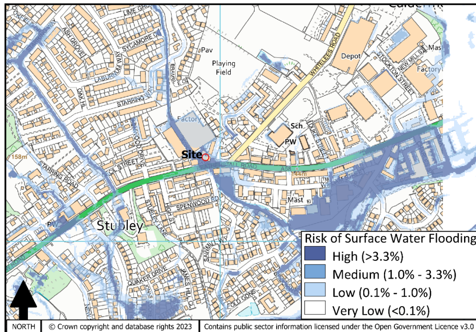
Figure 4.1 Surface Water Flooding Extents
