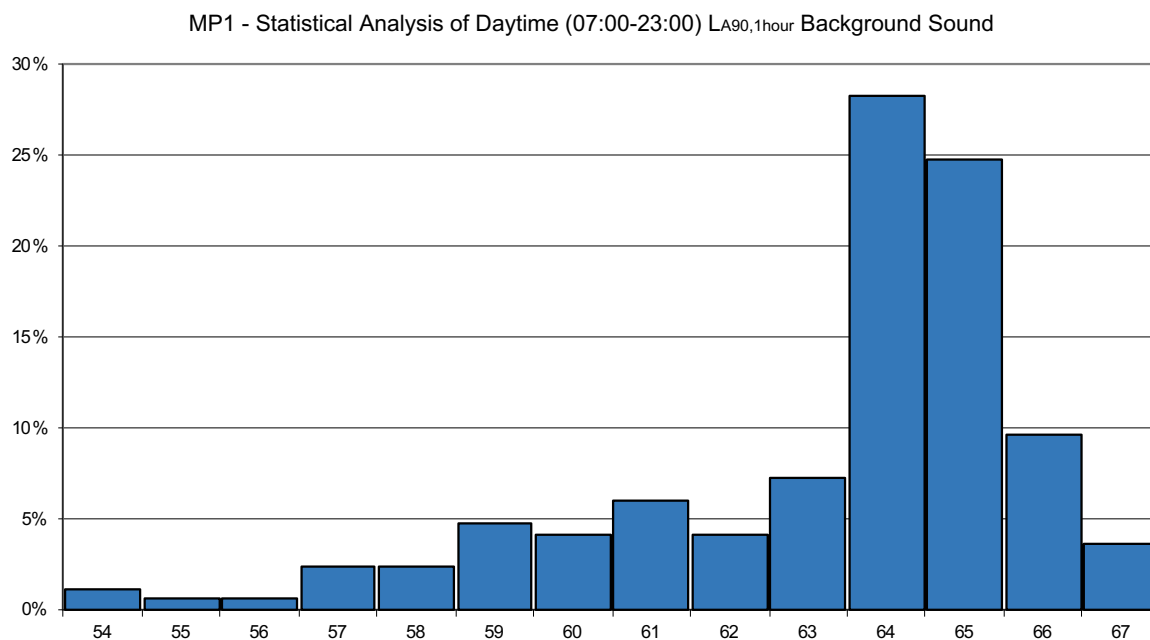
FIGURE 6: STATISTICAL ANALYSIS OF L_{A90} BACKGROUND – DAYTIME – MP1
