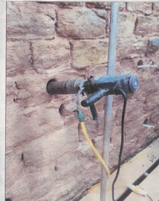
2. CINTEC TIES
