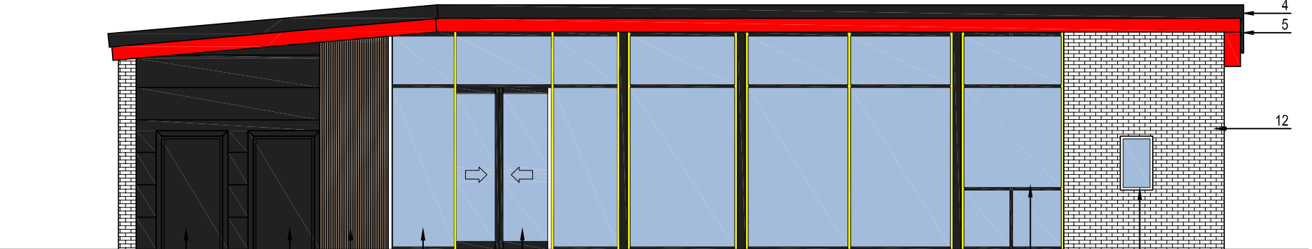
NORTHEAST ELEVATION
