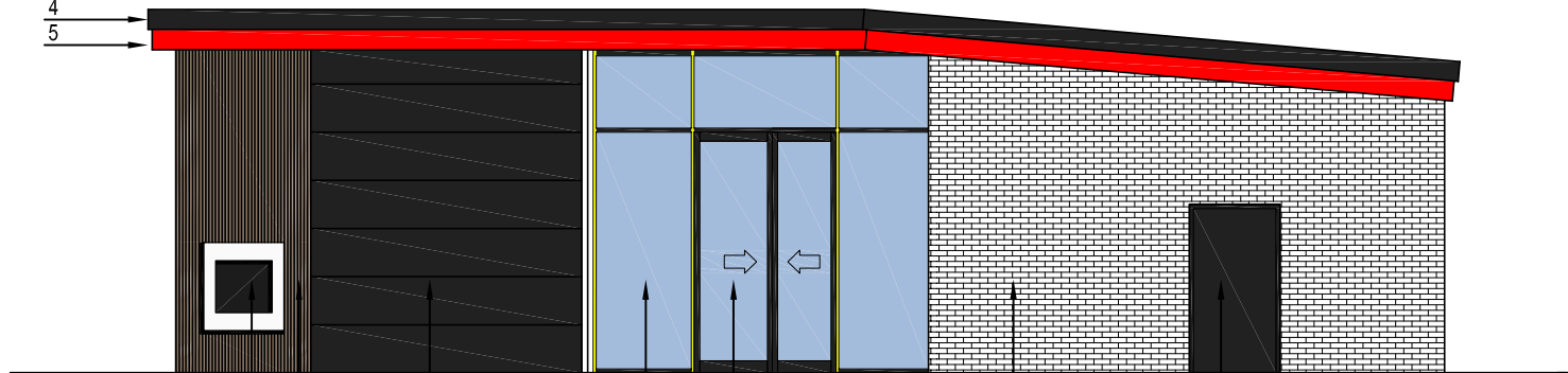
NORTHWEST ELEVATION
