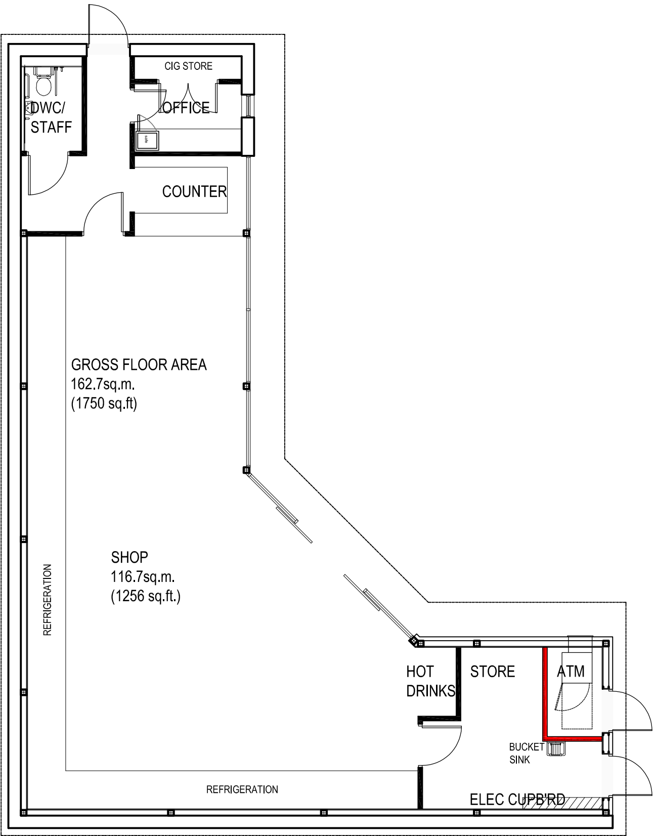
FLOOR PLAN AS PROPOSED
