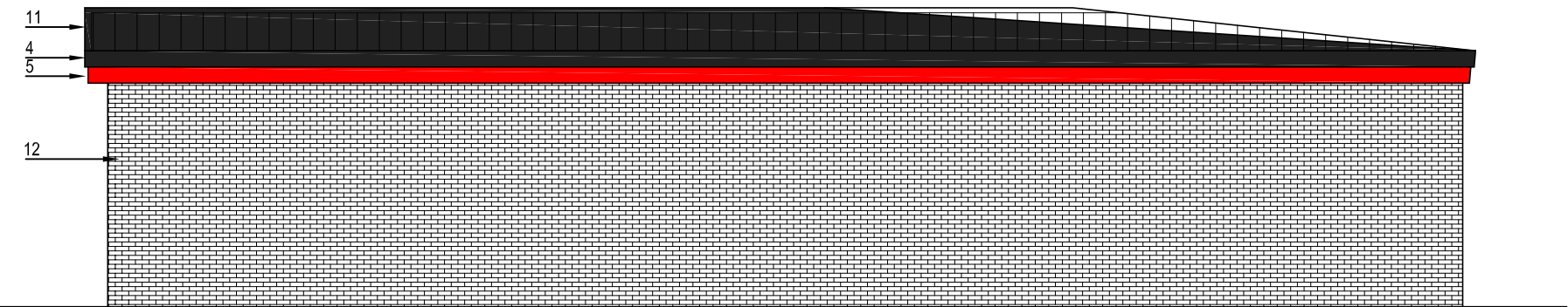
SOUTHWEST ELEVATION
