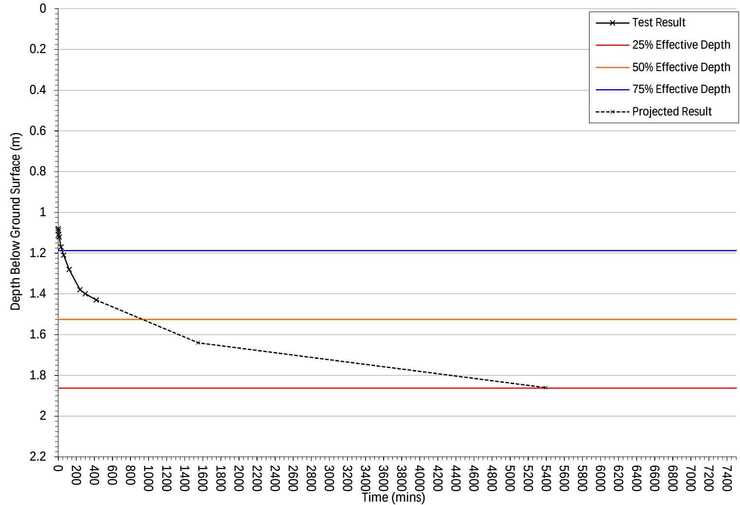
Results of Field Observations 6127 VGHM TP12 Soakaway Test 17th Aug 2023
