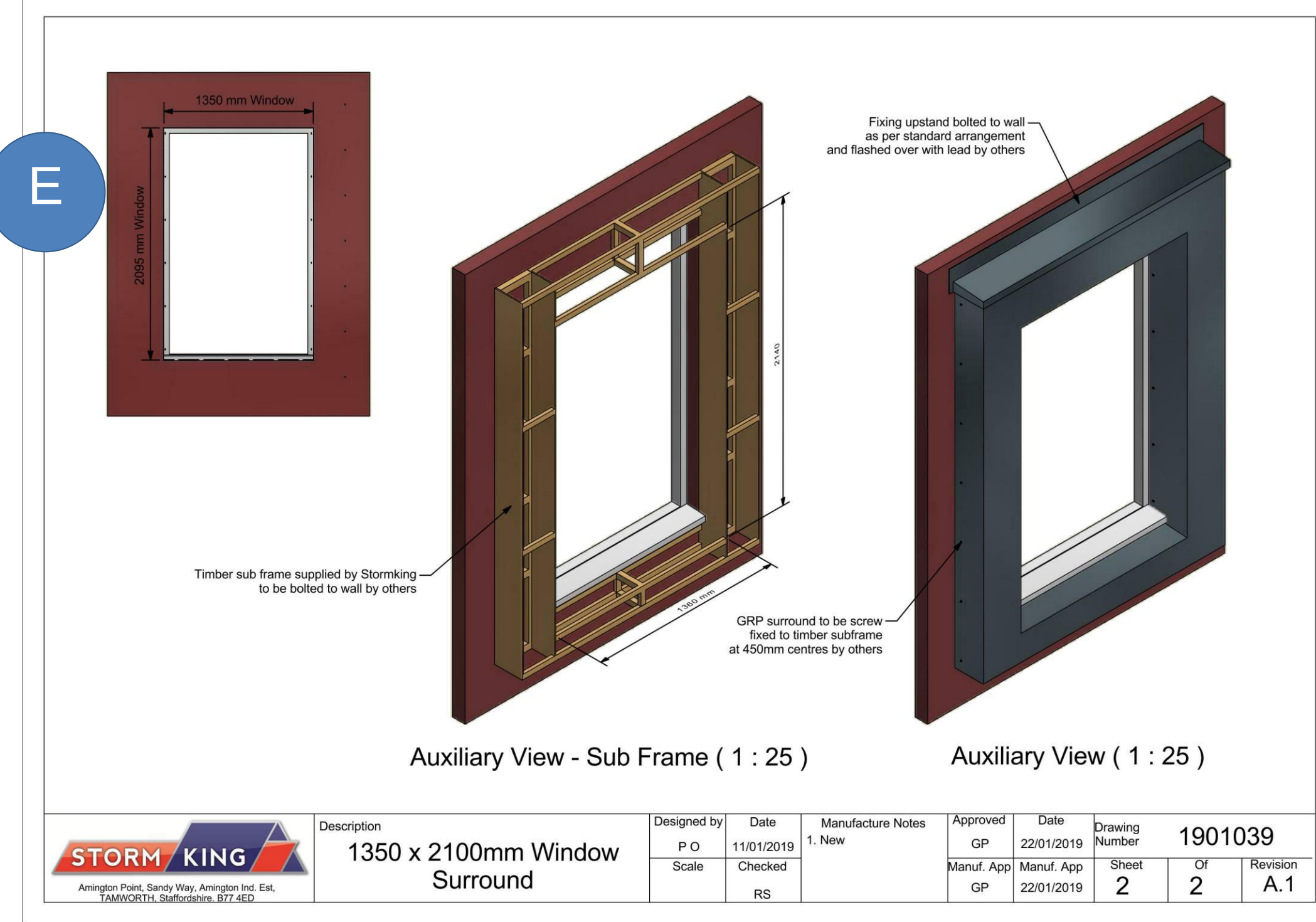
GRP preformed window feature
