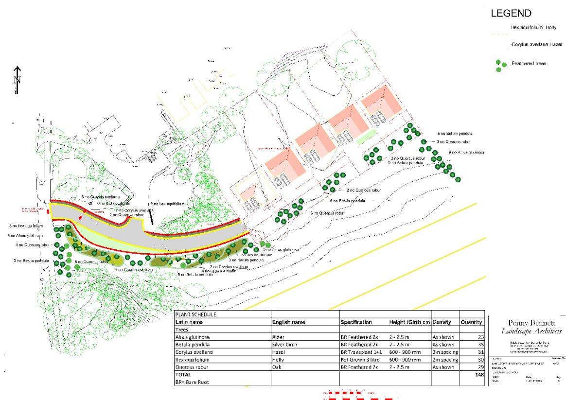
Figure 1 Site plan
