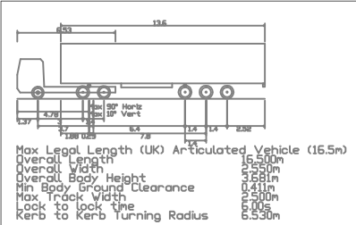
SWEPT PATH ANALYSIS - 16.5M ARTICULATED HGVS TURNING IN AND OUT FROM THE IMPROVED ACCESS ROAD - 1:1000
