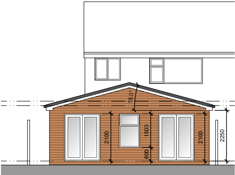
East Facing Rear Elevation
