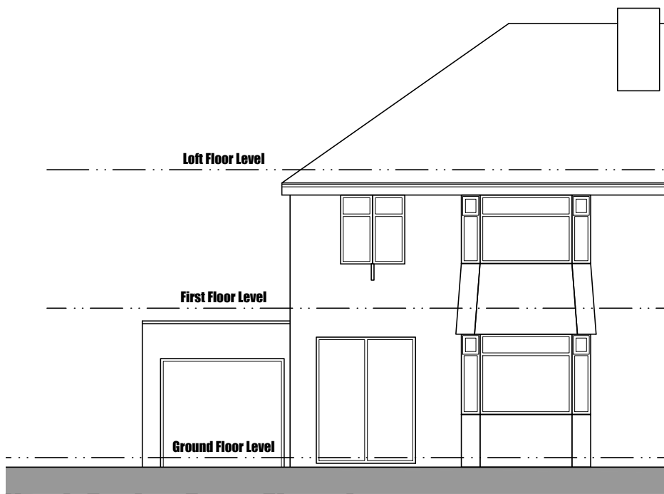
North Facing Front Elevation
