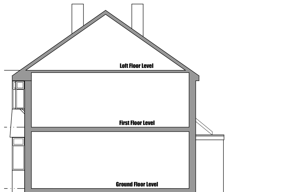
West Facing Side Elevational Section
