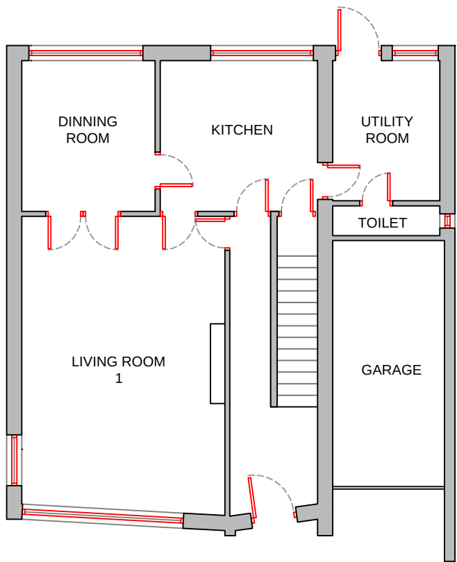
EXISTING GROUND FLOOR 1:100
