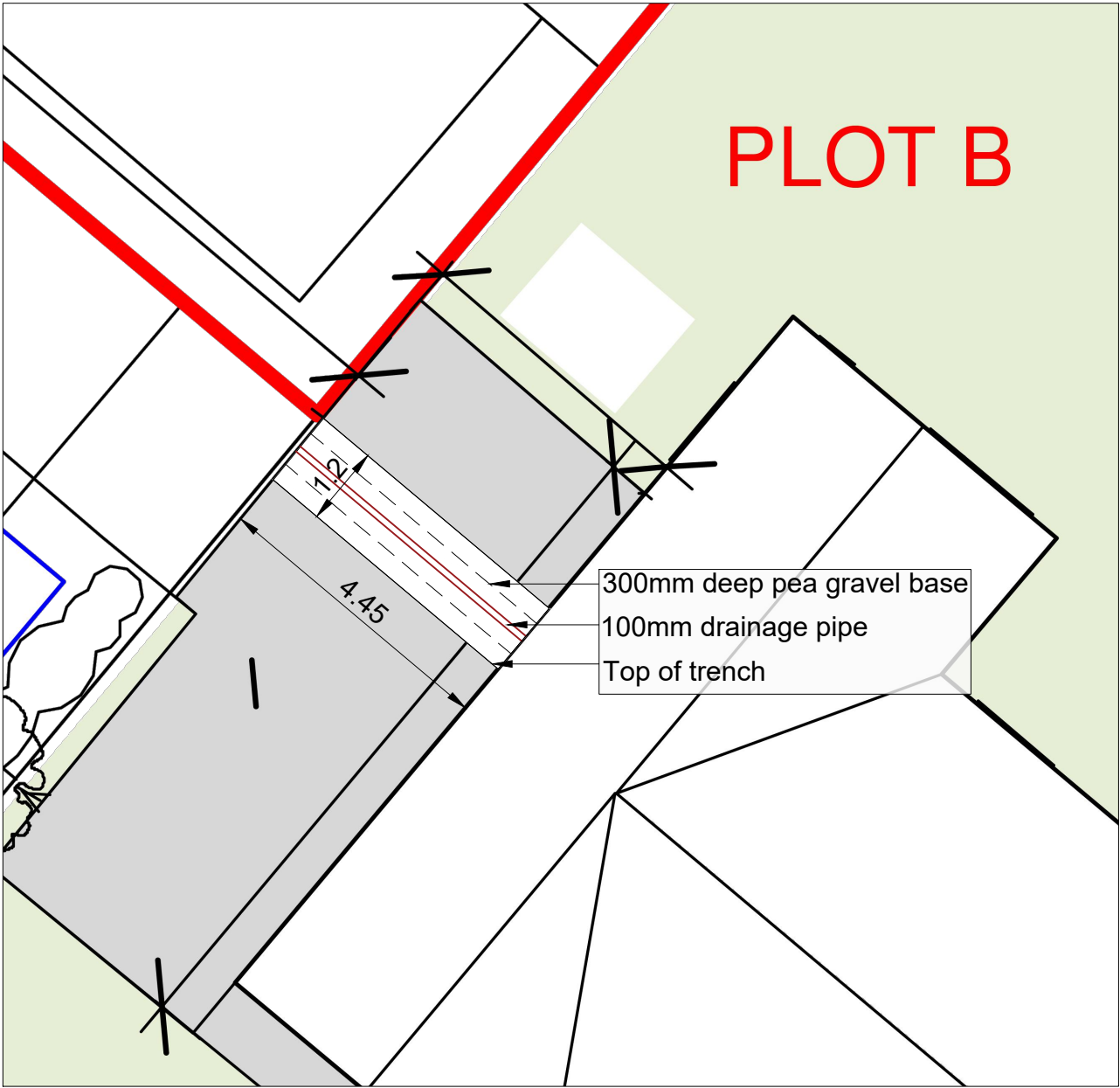
Plan (1:100)
