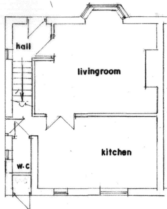
G.F. PLAN (EXISTING)
