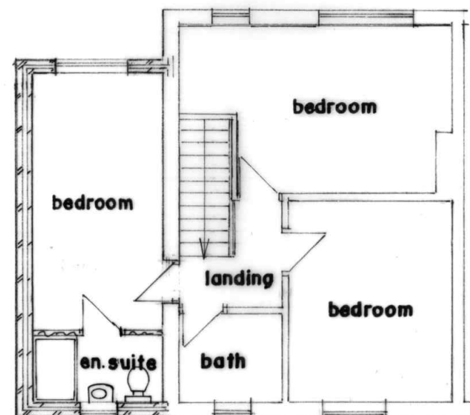
FIRST FLOOR PLAN (PROPOSED)
