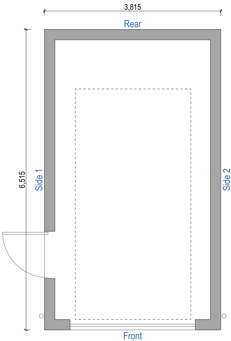
Garage - Floor Plan 1:50
