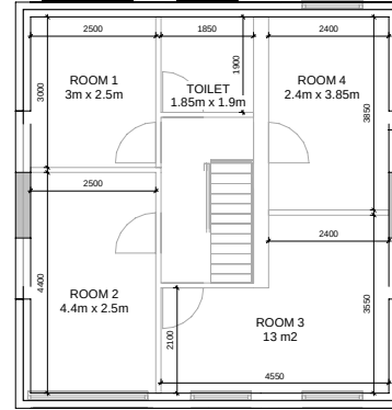
5 LEVEL 2 1:50
