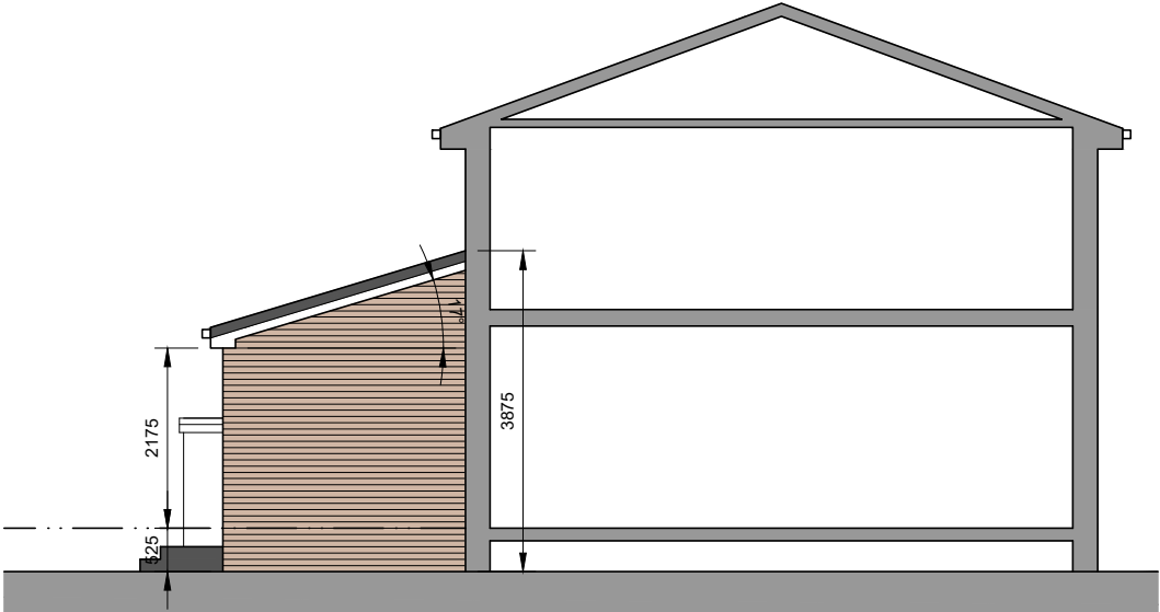
East Facing Side Elevation
