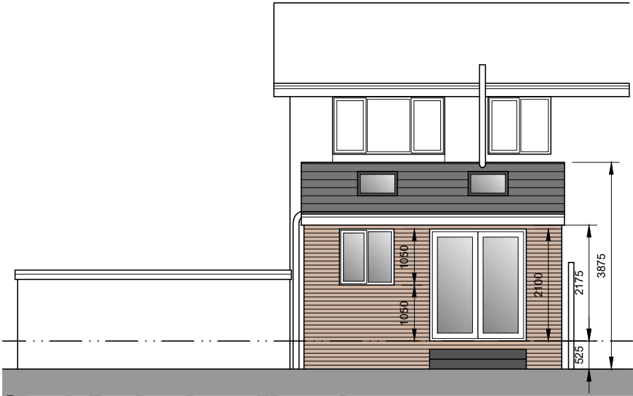
South Facing Rear Elevation
