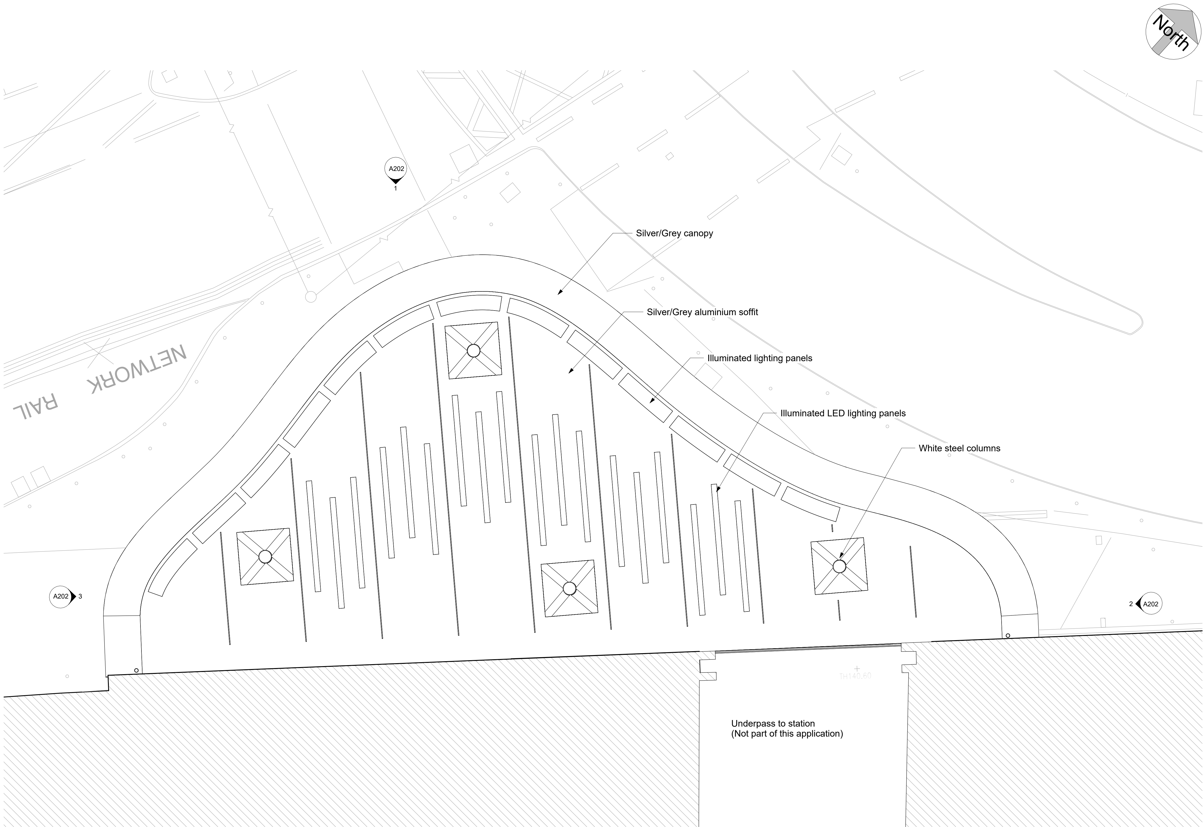
2 Forecourt Works - Roof Soffit Plan 1 : 50
