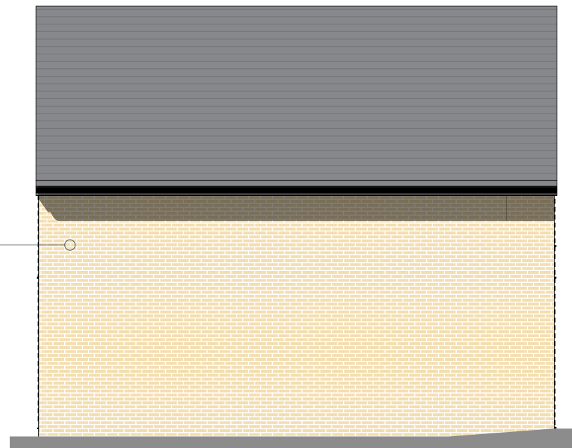
Side 1 Elevation 1:100
