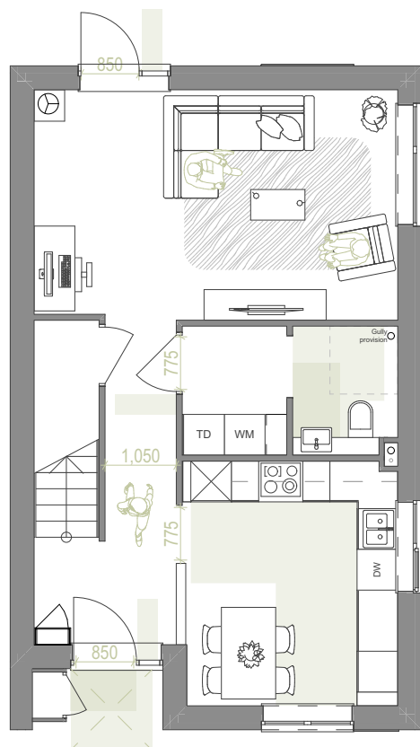
Ground Floor 1:100
