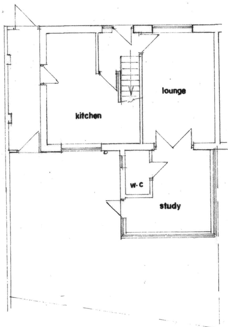
GROUND FLOOR PLAN (EXISTING)
