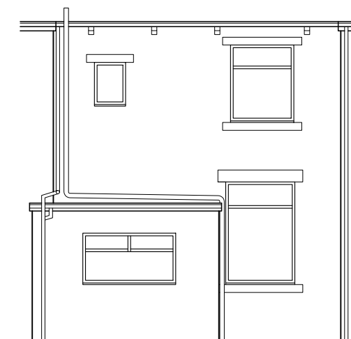
EXISTING REAR ELEVATION - 1:100
