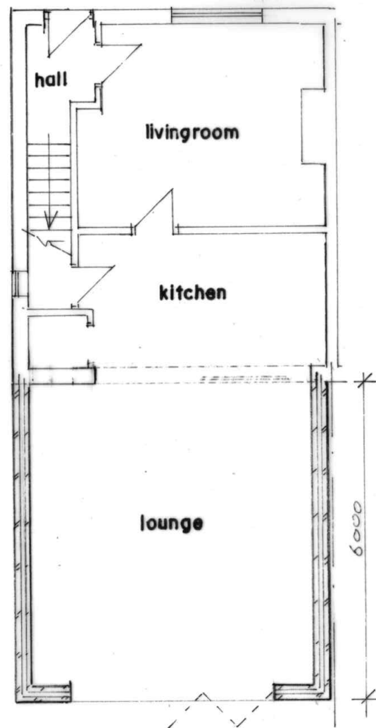
GROUND FLOOR PLAN (PROPOSED)
