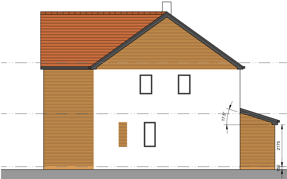
North Facing Side Elevation
