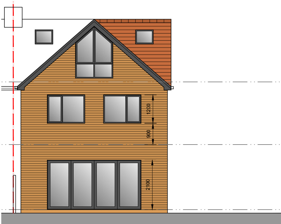
East Facing Rear Elevation
