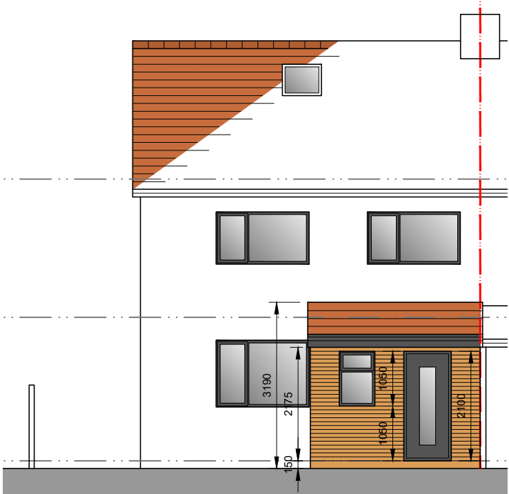
West Facing Front Elevation
