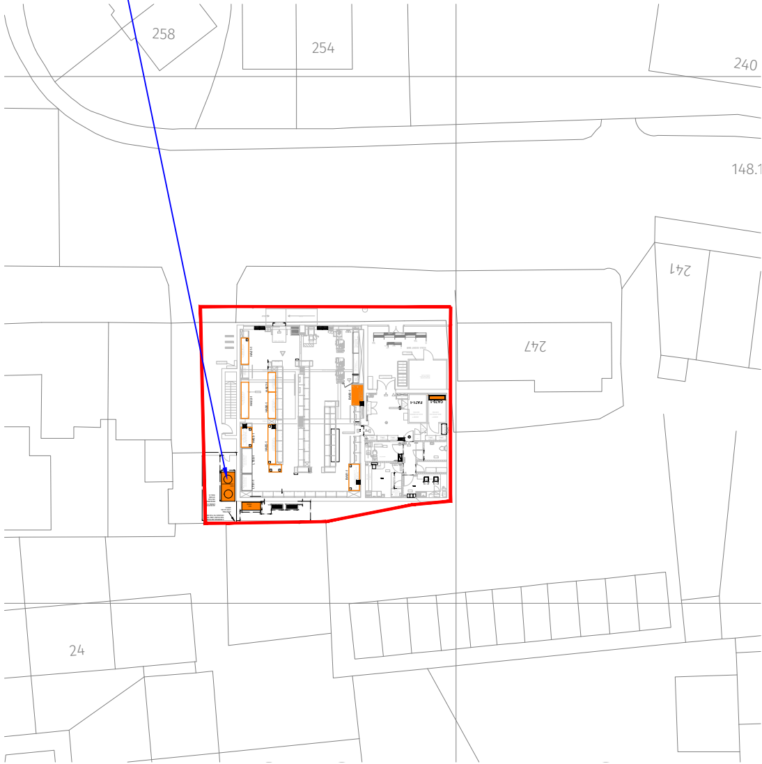
2 PROPOSED SITE PLAN 1:500
