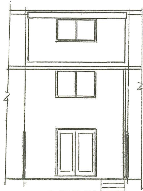
EXISTING REAR ELEV
