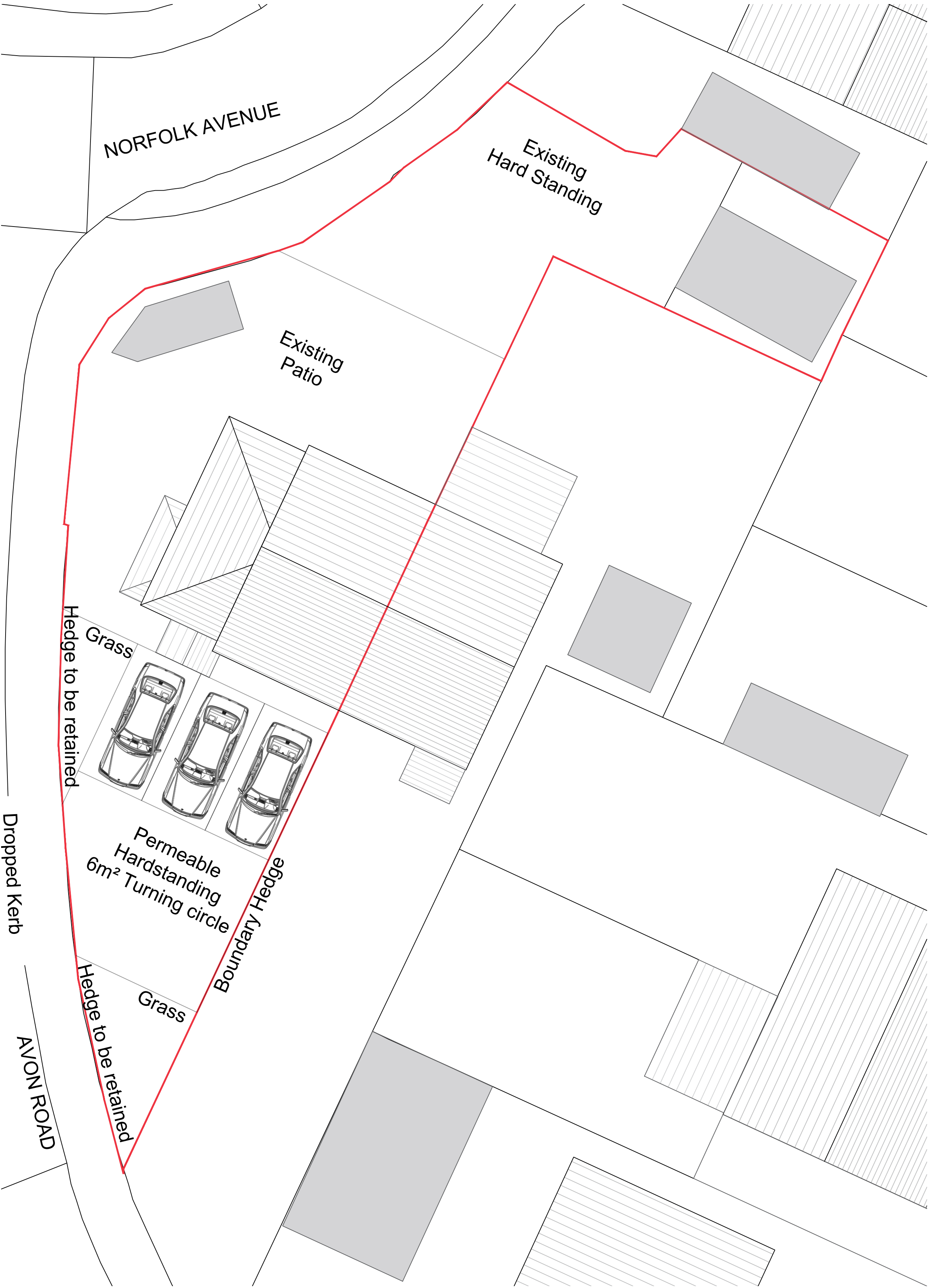
Proposed Roof and Block Plan 1:100 Scale @ A1 1:200 Scale @ A3
