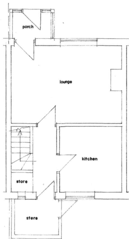
G.F. PLAN (EXISTING)
