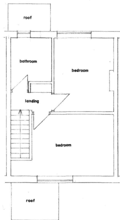
F.F. PLAN (EXISTING)
