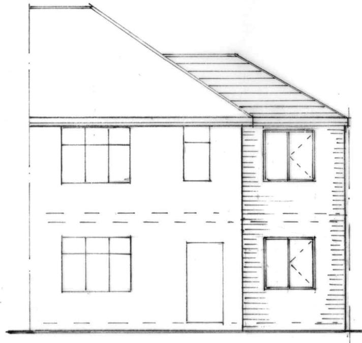
FRONT ELEVATION (PROPOSED)
