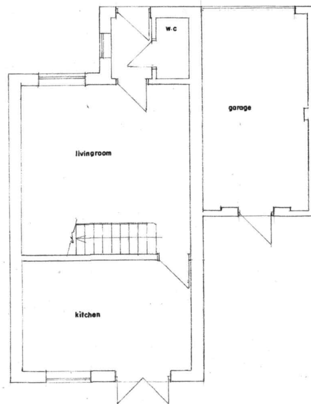
G. F PLAN (EXISTING)
