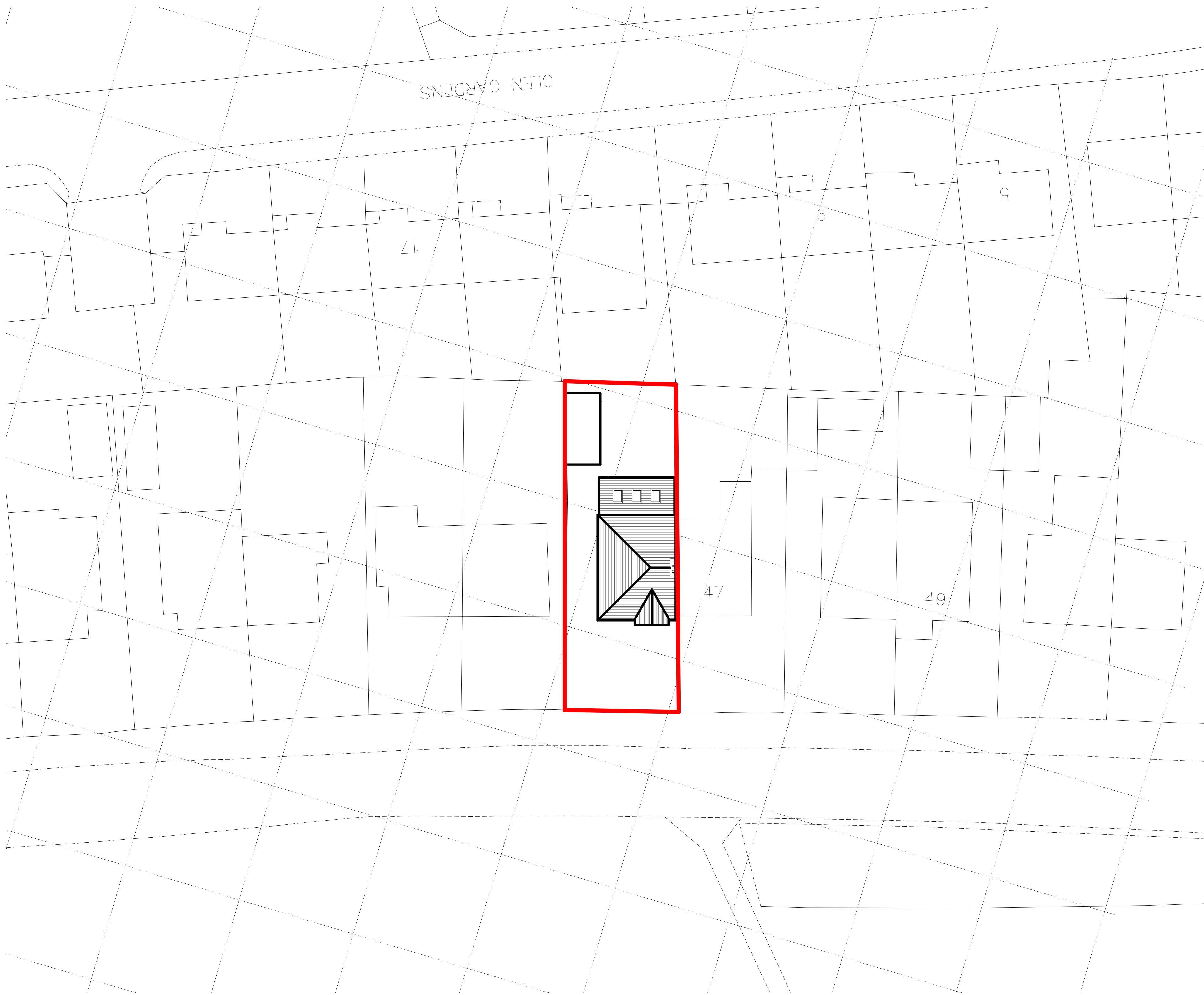
1 Proposed Site Plan 1 : 200
