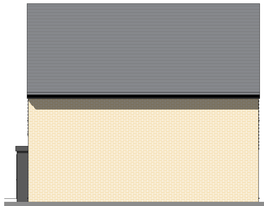
Side 2 Elevation 1:100
