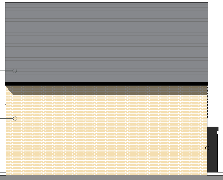
Side 1 Elevation 1:100
