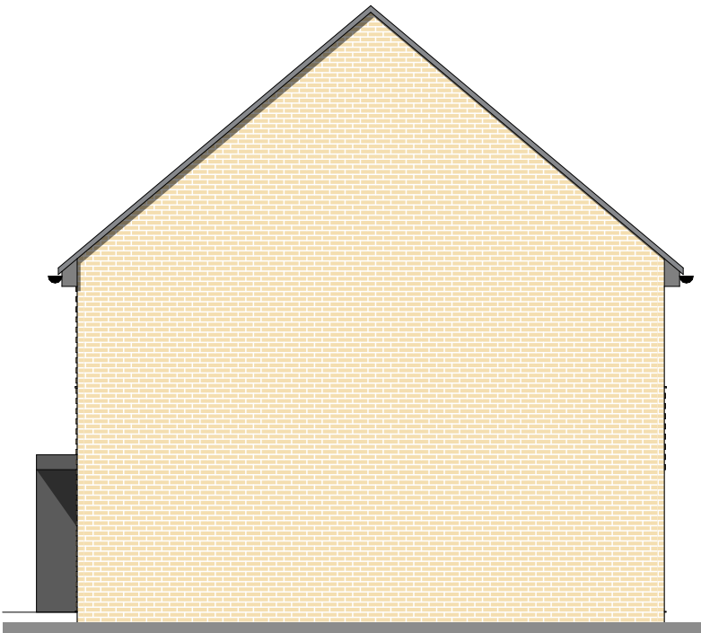
Side 2 Elevation 1:100
