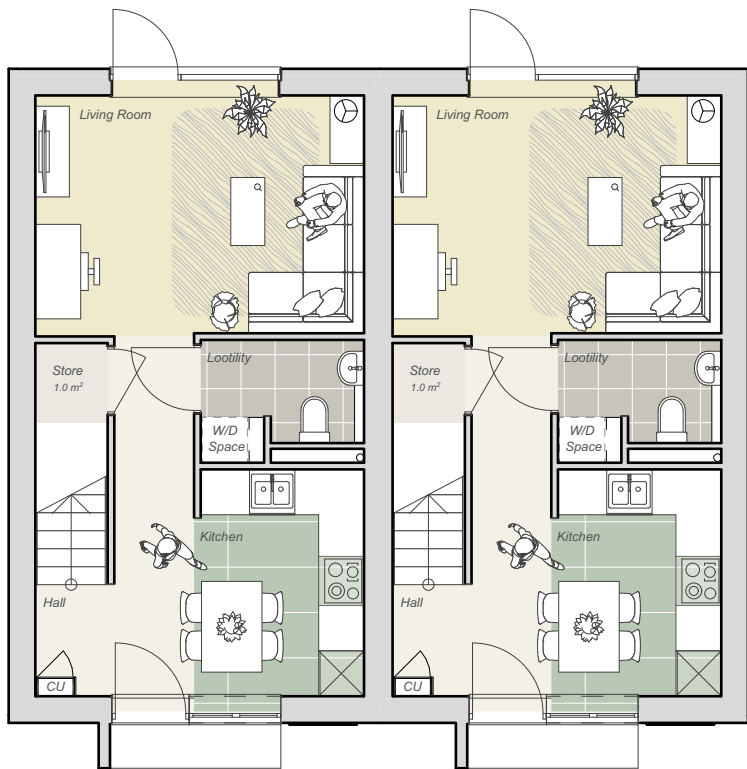
Ground Floor 1:100
