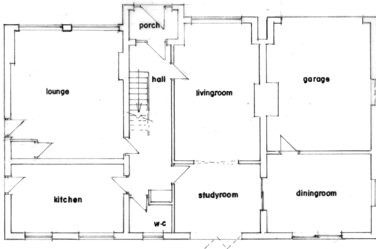
GROUND FLOOR PLAN (PROPOSED)
