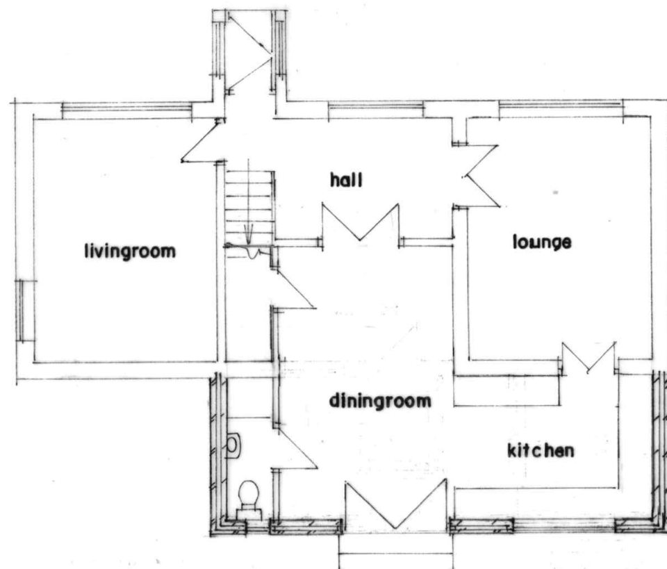
GROUND FLOOR PLAN (PROPOSED)
