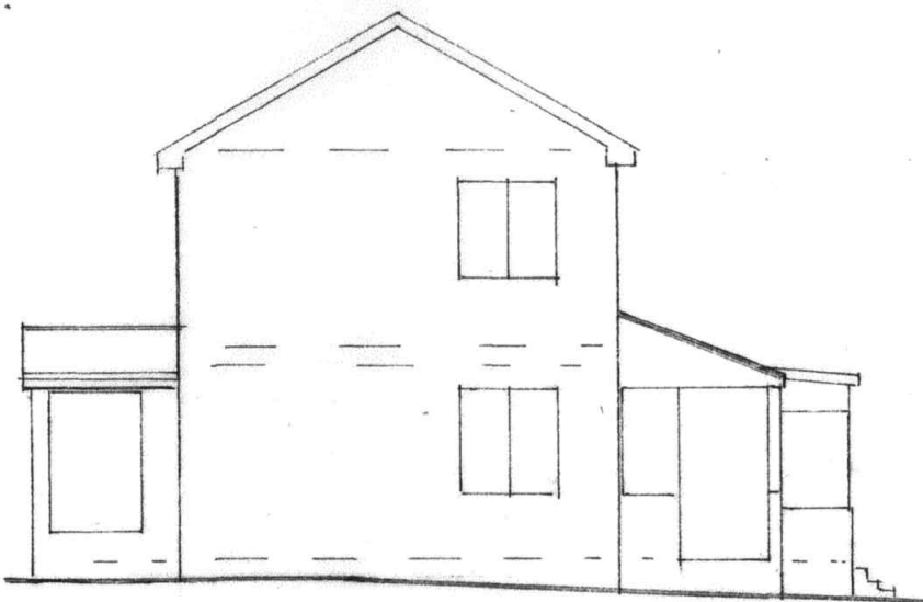
SIDE ELEVATION (EXISTING)
