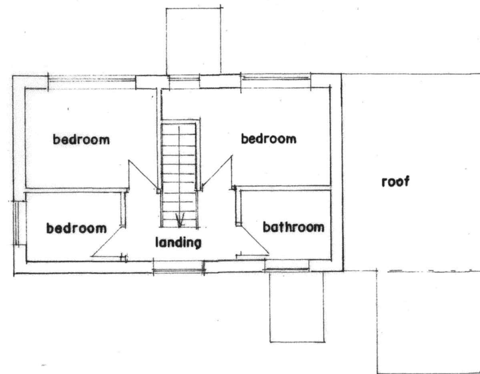
F.F. PLAN (EXISTING)
