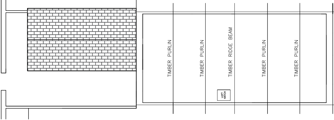
EXISTING LOFT FLOOR PLAN
