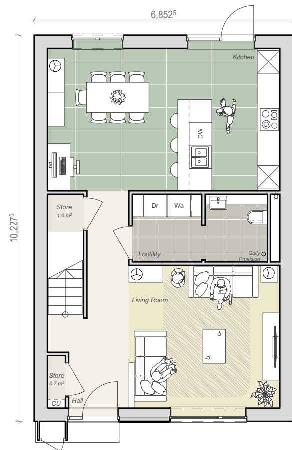
Ground Floor 1:100
