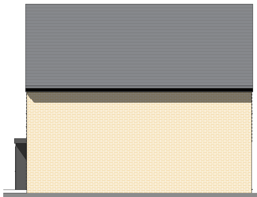
Side 2 Elevation 1:100
