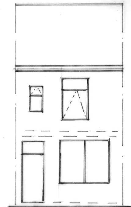
FRONT ELEVATION (PROPOSED)
