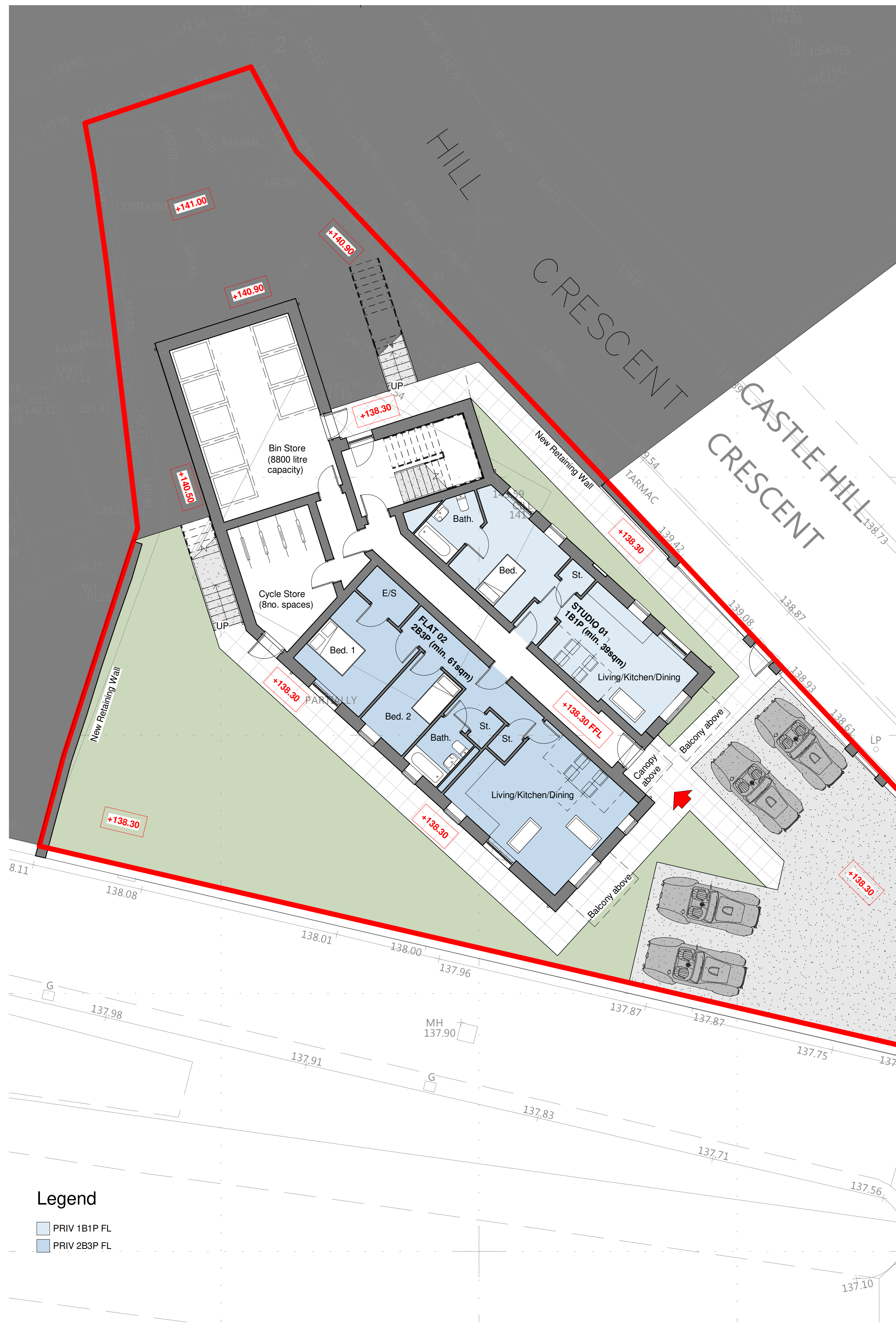
1 Proposed Level 0 1 : 100
