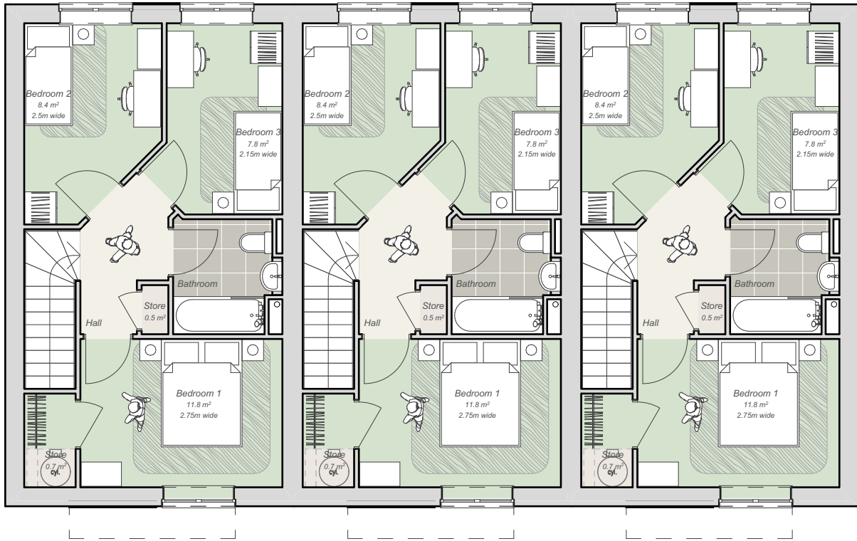
First Floor 1:100
