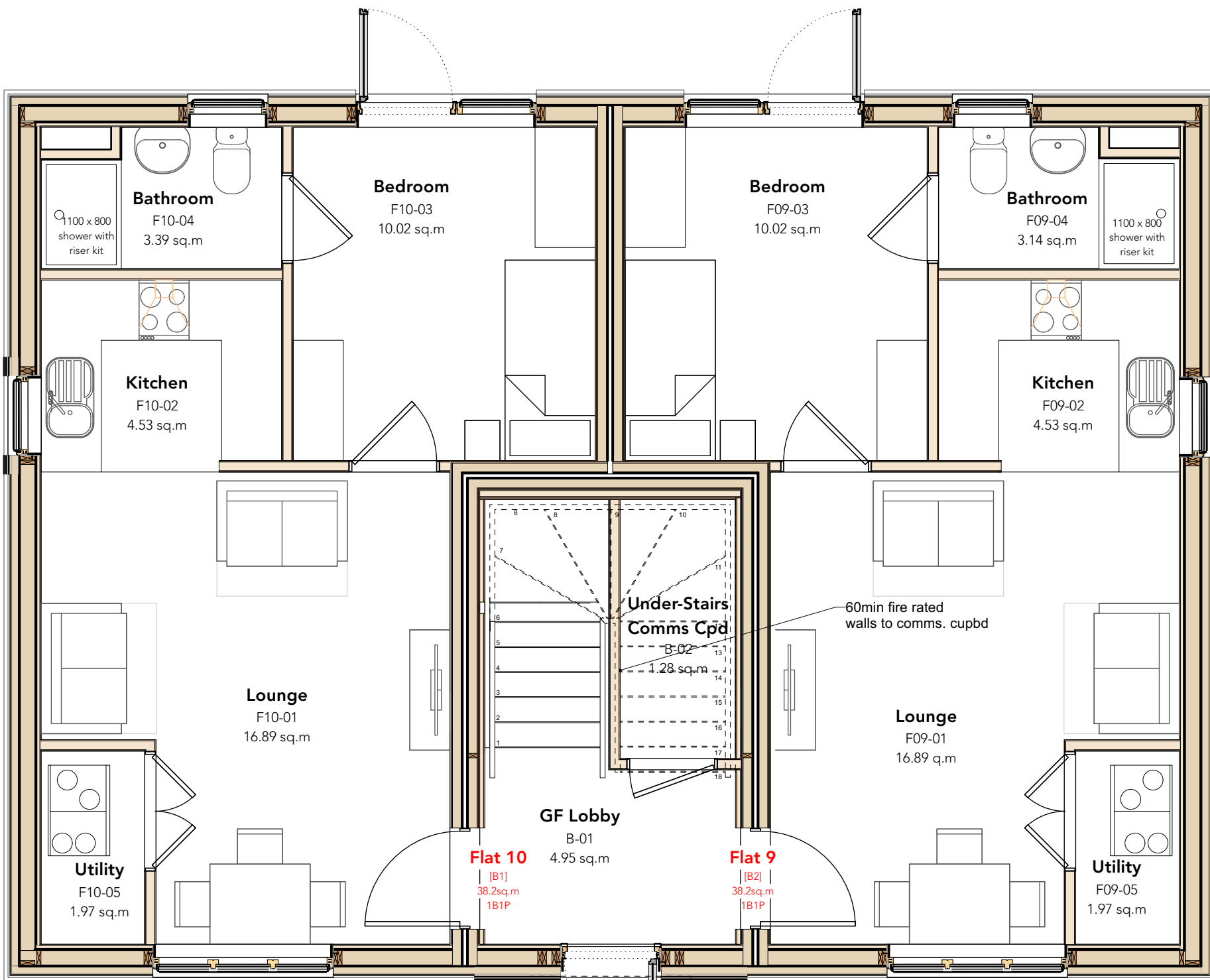
01 Block B - GF (L0)
