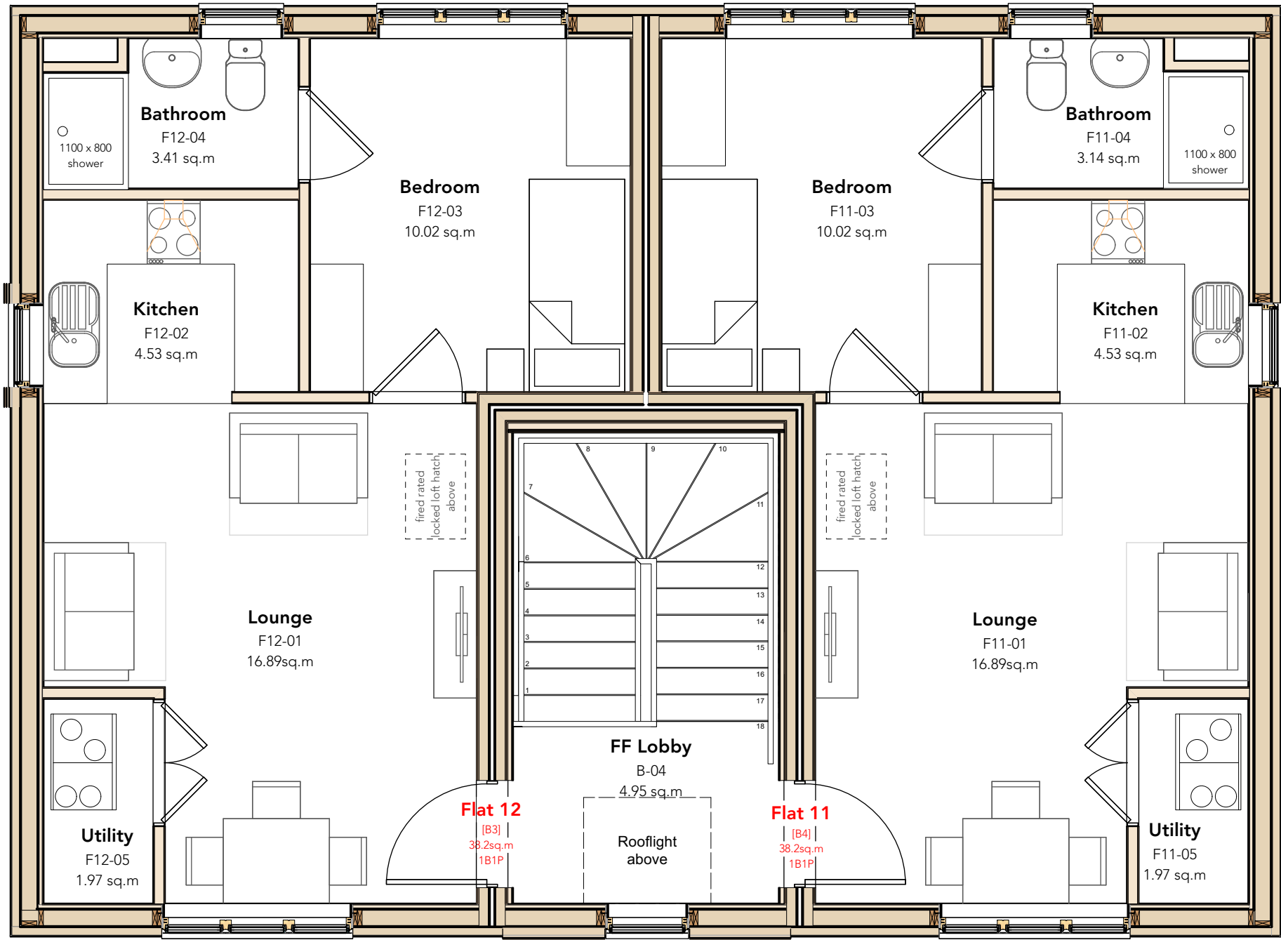
02 Block B - FF (L1)
