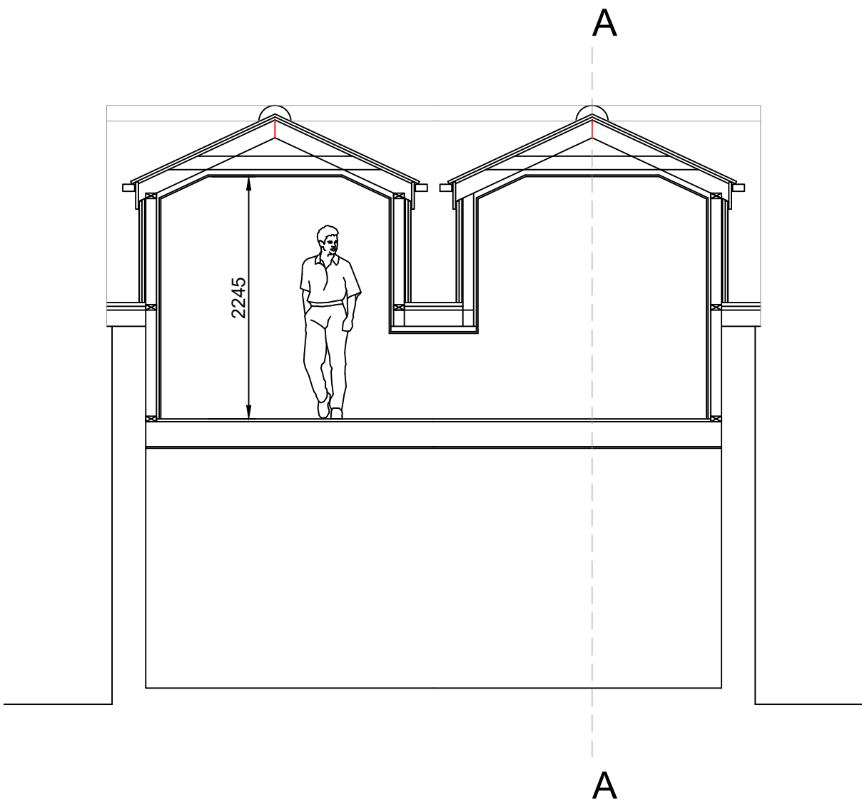
PROPOSED CROSS SECTION BB scale 1 - 50
