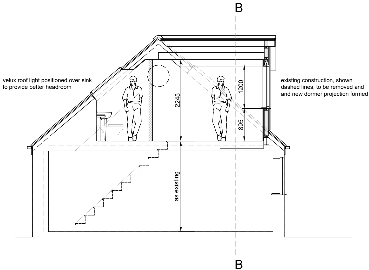
PROPOSED CROSS SECTION AA scale 1 - 50
