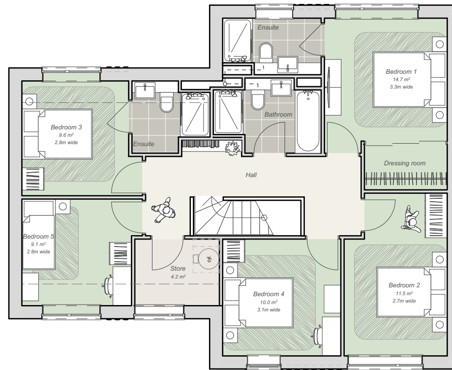
First Floor 1:100
