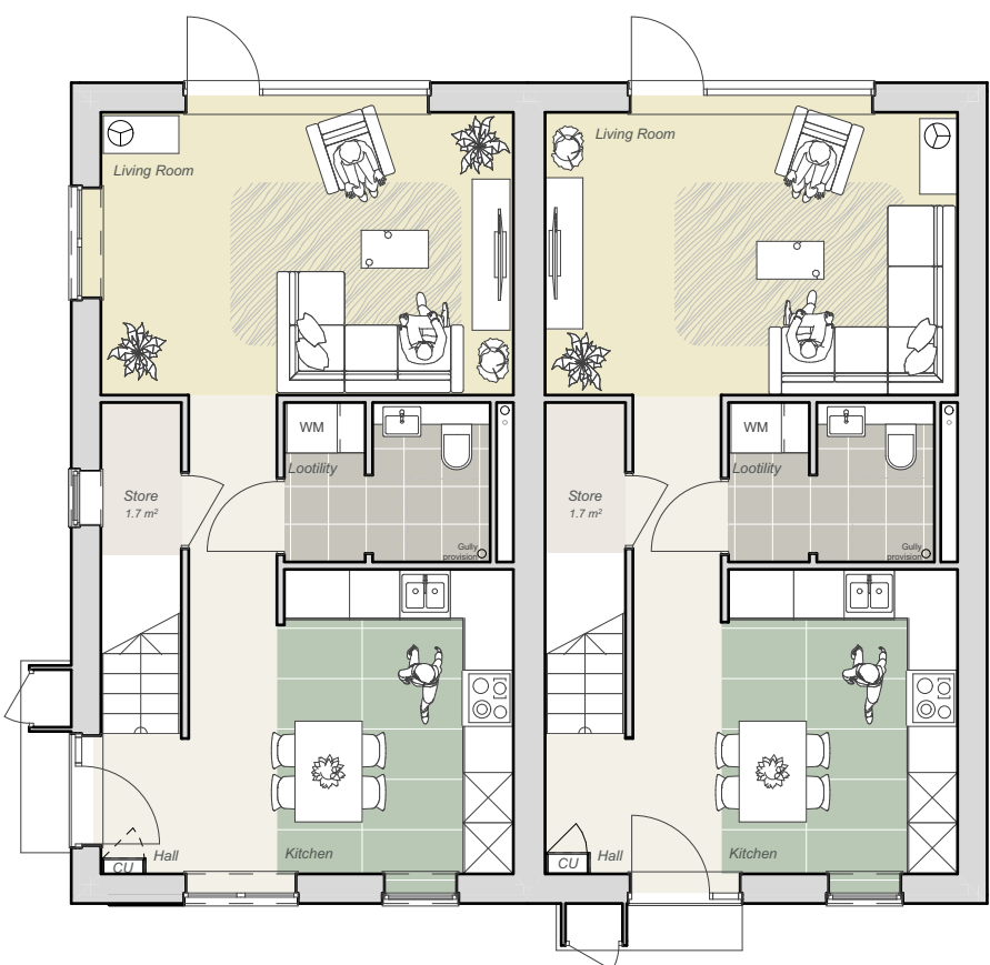
Ground Floor 1:100
