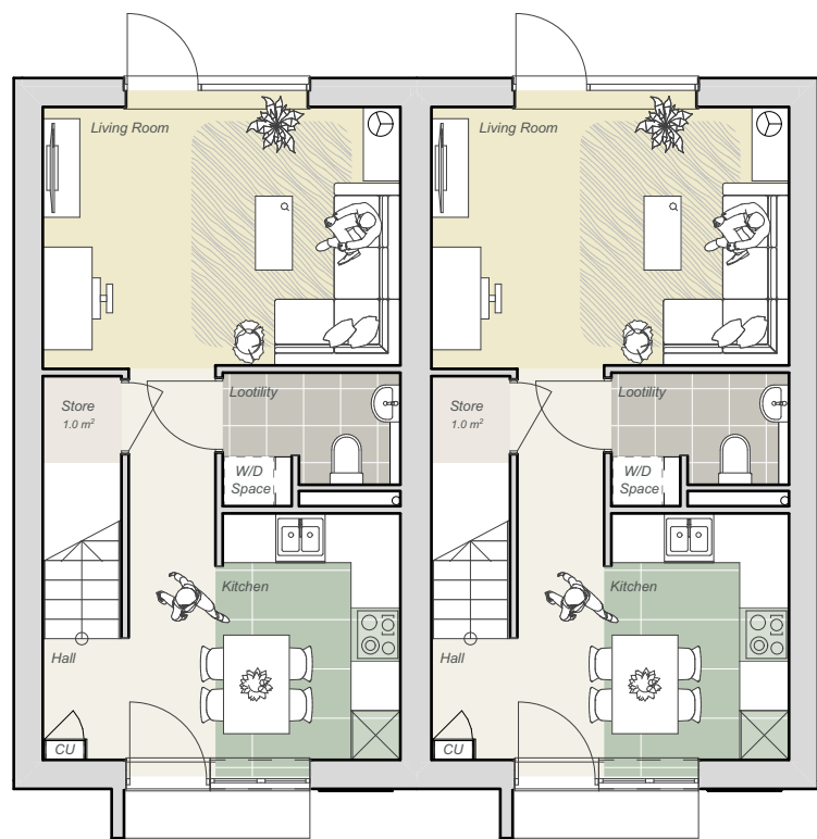
Ground Floor 1:100
