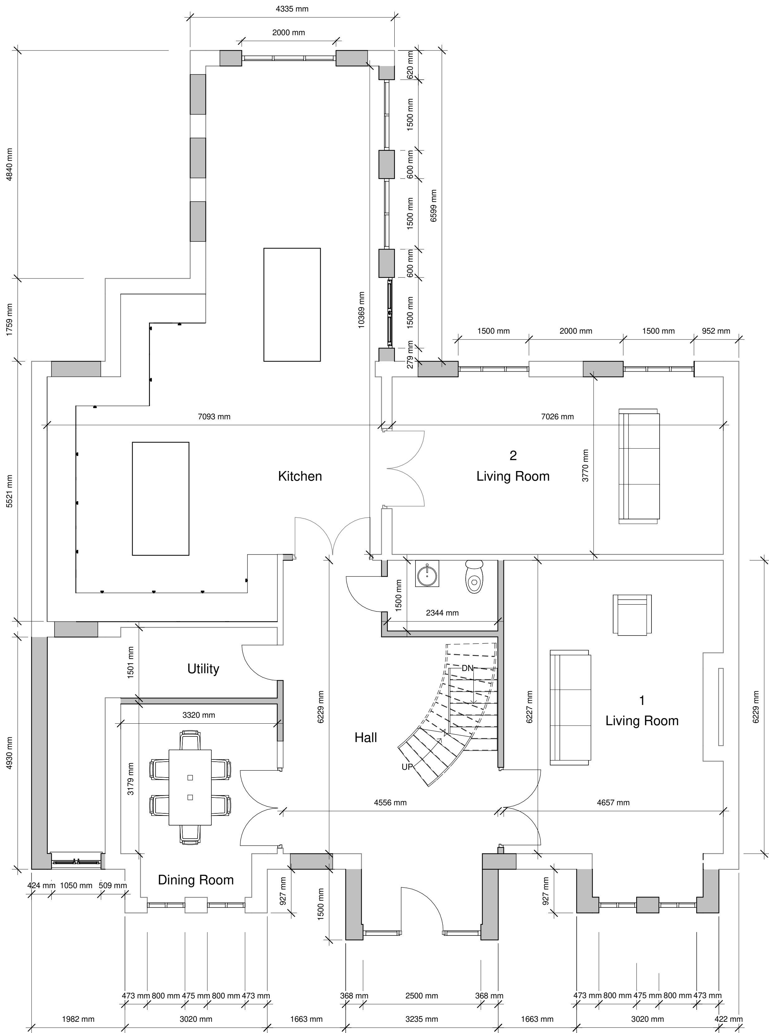
1 Ground Floor - Proposed 1 : 50
