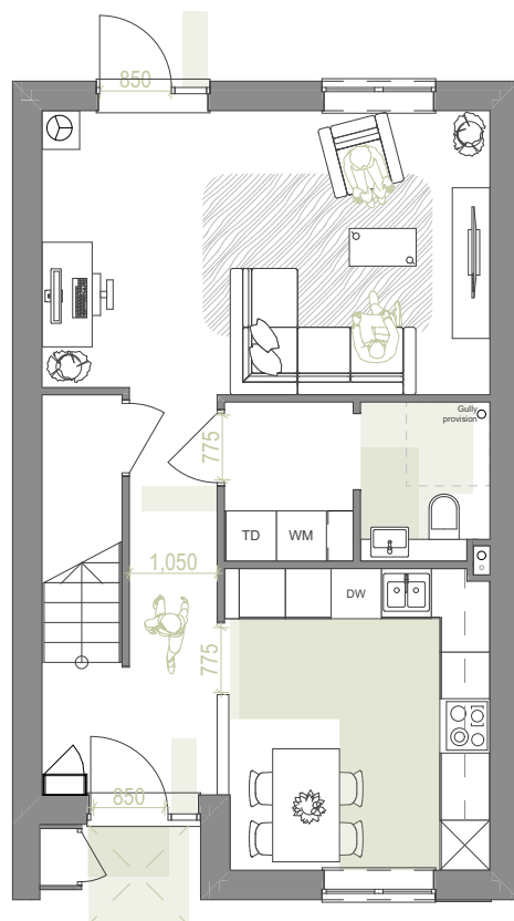
Ground Floor 1:100
